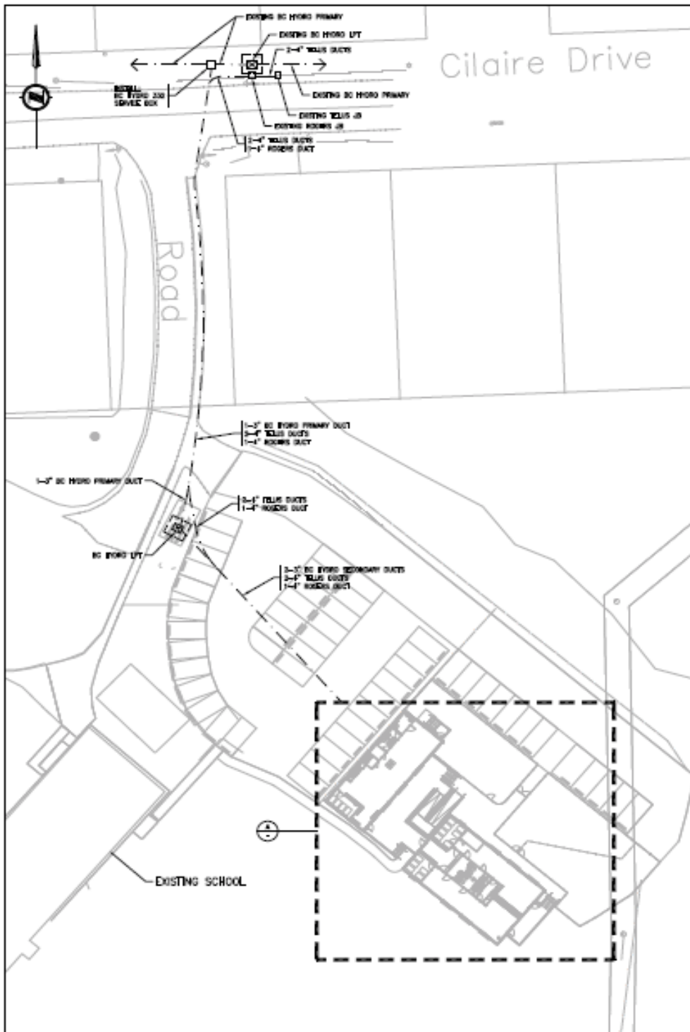
OVERALL SITE PLAN SCALE: 1:500
